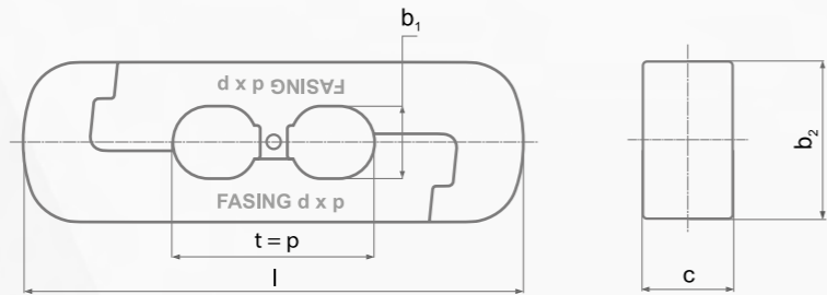
Dimensions and mechanical properties - OZBR for Solid Profile
